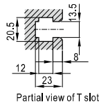
Partial view of T slot
